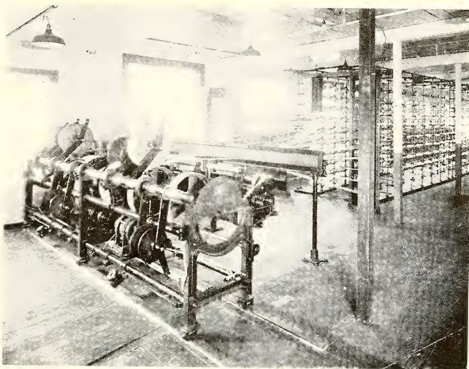
Machinery Made in Gastonia Finds a Market Throughout the Civilized World.
