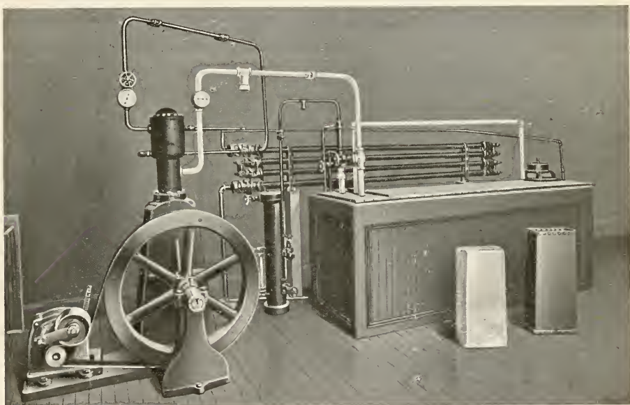
A SMALL ICE-MAKING PLANT
